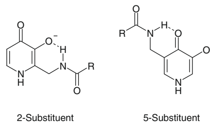
Figure 1. Intramolecular H-bond formation in ortho amido-3-hydroxypyridin-4-ones.
