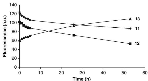
Figure 6. Competition of iron(III) between transferrin and hexadentate probes 11 , 12 and 13 . Monoferrous transferrin (65 \mu\text{M} ) was prepared from apotransferrin and \text{Fe}(\text{NTA})_2 , both the final concentration at 65 \mu\text{M} , in \text{NaHCO}_3 (50 mM, pH 8.0) and the solution was incubated at 37 ^\circ\text{C} for 1 h before use. Half-full iron-chelated probes (12 \mu\text{M} ) was prepared from fluorescent probes (12 \mu\text{M} ) and \text{Fe}(\text{NTA})_2 (6 \mu\text{M} ) in MOPS (50 mM, pH 7.4). Equal volumes of mono-transferrin and half-full iron-chelated probes were mixed and the fluorescence was measured immediately and continually at 435/474 nm excitation/emission using a spectrofluorometer for 53 h.
